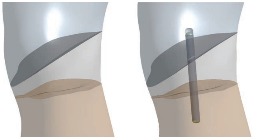
▲ Finite element submodels of Adam's left knee. Left: adhesive-only join. Right: fiberglass pin from thigh, through wedge, to calf. The pin in this model is larger than the one ultimately used in the sculpture.
