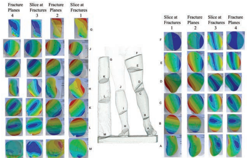
▲ Adam's tree trunk along with right and left legs (center), with ANSYS Mechanical stress results on either side. Columns 1 and 2 illustrate compressive (represented by blue and green) and tensile (represented by orange and red) stresses. Columns 3 and 4 illustrate shear stress.
